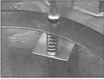
Install the lamp base with three springs and the 1-1/2" screws.
